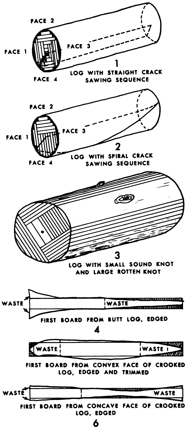
Figure 9-1. Sawing procedures.
